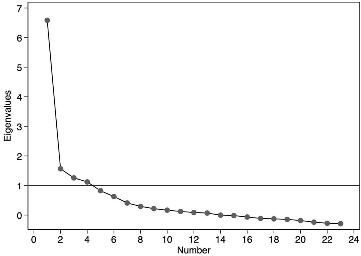
Figure A1. Scree plot of eigenvalues after factor
